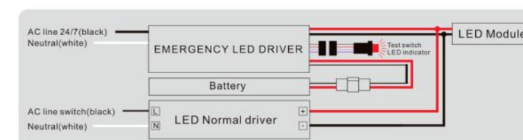
Wiring Diagram for Serial Numbers 1-8
