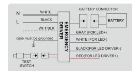
Wiring Diagram for Serial Numbers 9-12
